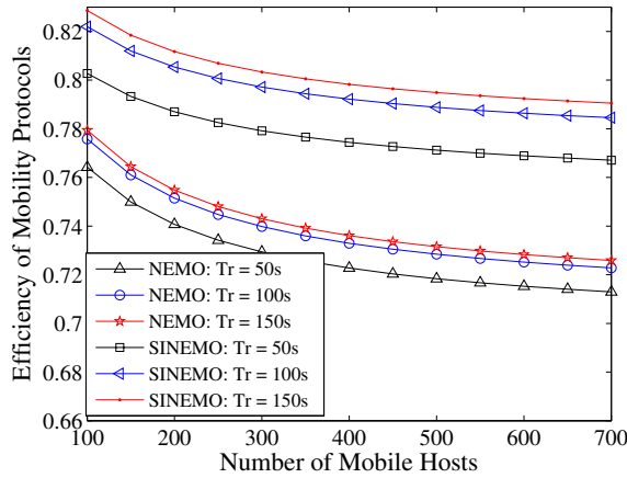
Fig. 5. Efficiency of SINEMO and NEMO vs. number of MHs for various subnet residence times.
