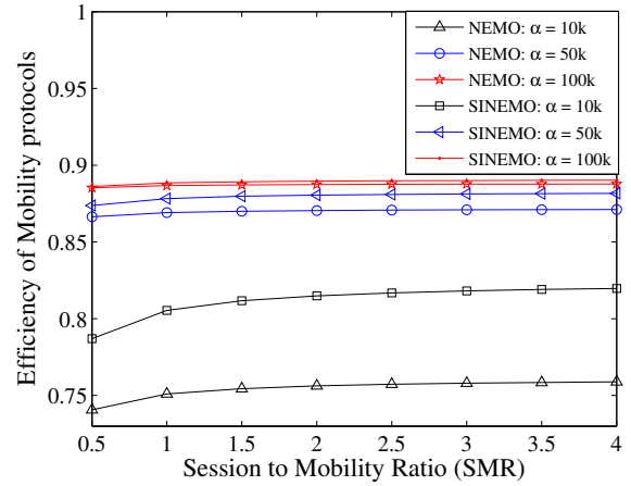
Fig. 6. Efficiency of SINEMO and NEMO BSP vs. SMR for various session lengths.
