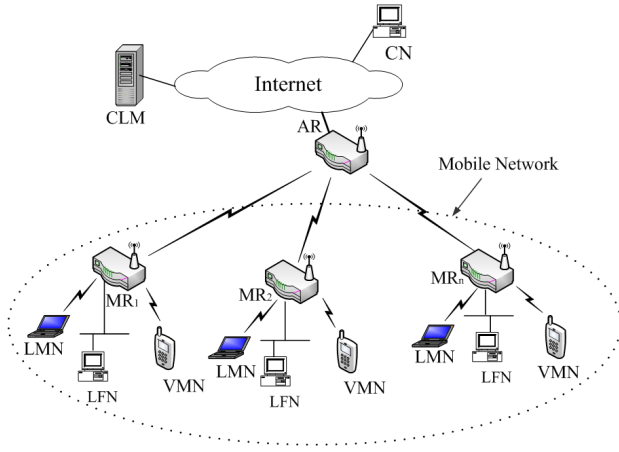
Fig. 1. SINEMO Architecture
