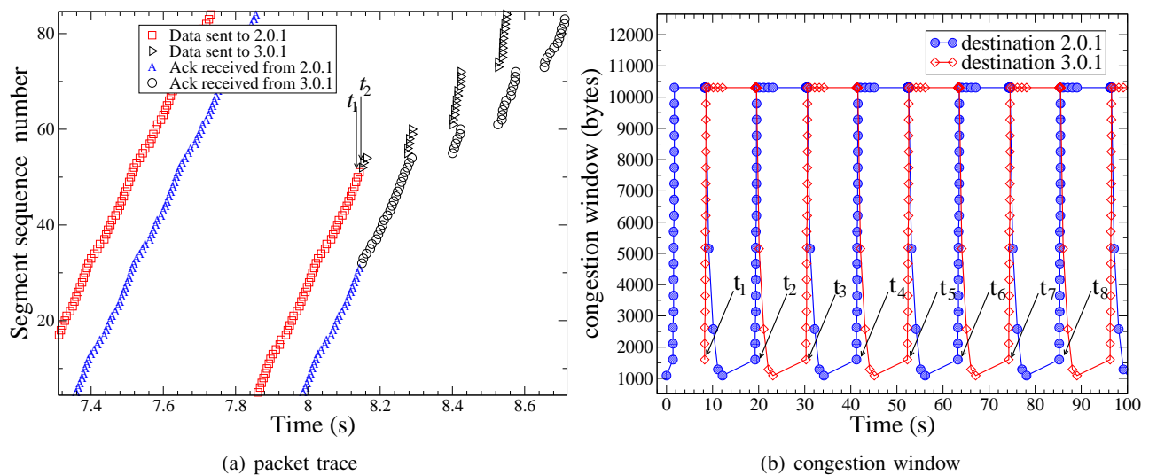
Fig. 11. Packet trace of SIGMA during one handover with no L2 handover latency.
