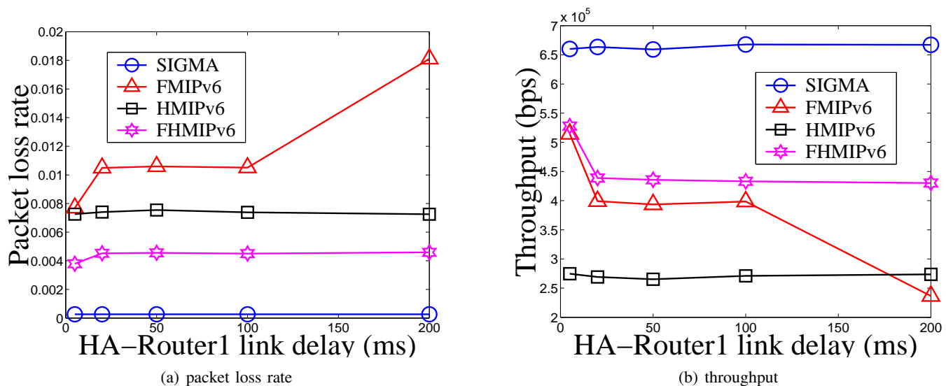
Fig. 15. Impact of HA-Router1 delay on packet loss rate and throughput.
