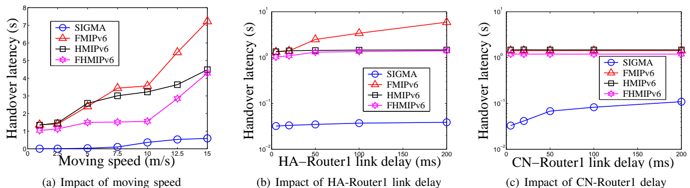
Fig. 13. Impact of different parameters on overall handover latency.
