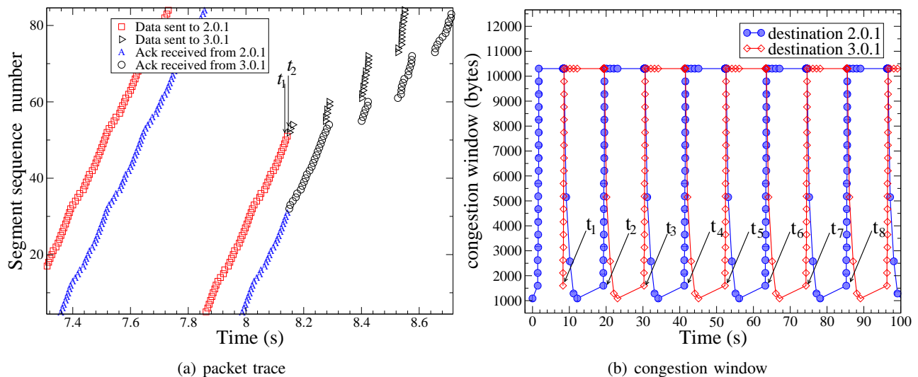
Fig. 12. Packet trace of SIGMA during one handover with 200ms L2 handover latency.
