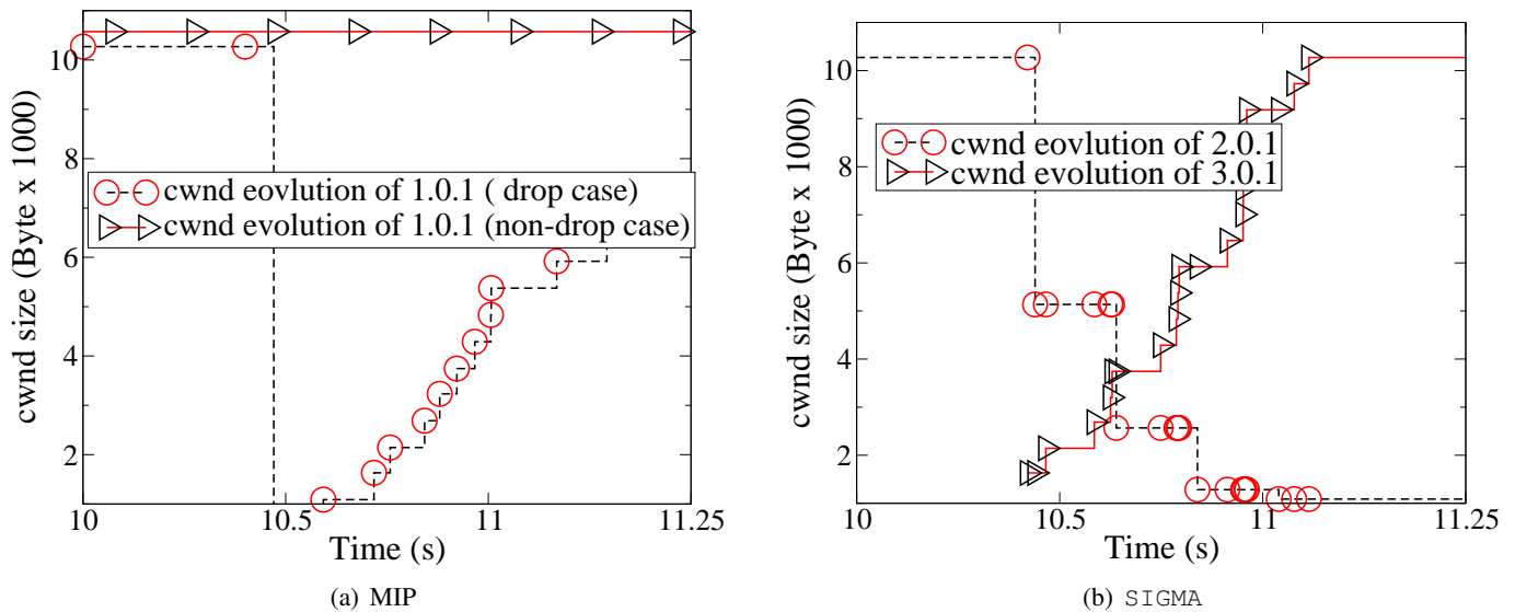
Fig. 17. cwnd evolution for MIP and SIGMA during handover.
