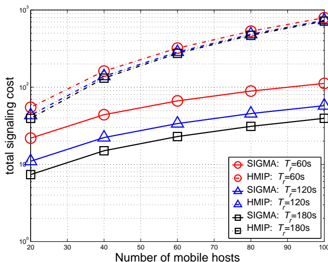
Fig. 6. Impact of number of MHs on total signaling cost of SIGMA and HMIPv6 under different subnet residence times.
