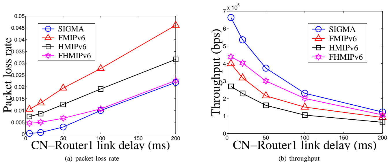
Fig. 16. Impact of CN-Router1 delay on packet loss rate and throughput.
