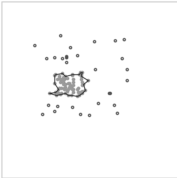
Fig.6 Alpha shape for clustering results of Model 4. Solid gray circles are those points satisfied the threshold and constrains.
