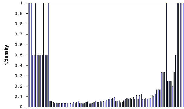
Fig.4 Cluster ordering of Model 4.
